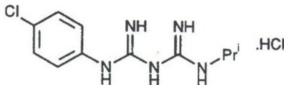
Proguanil Hydrochloride
